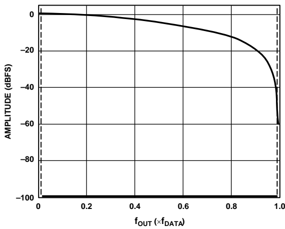
Figure 59. No Interpolation, Modulation Disabled
