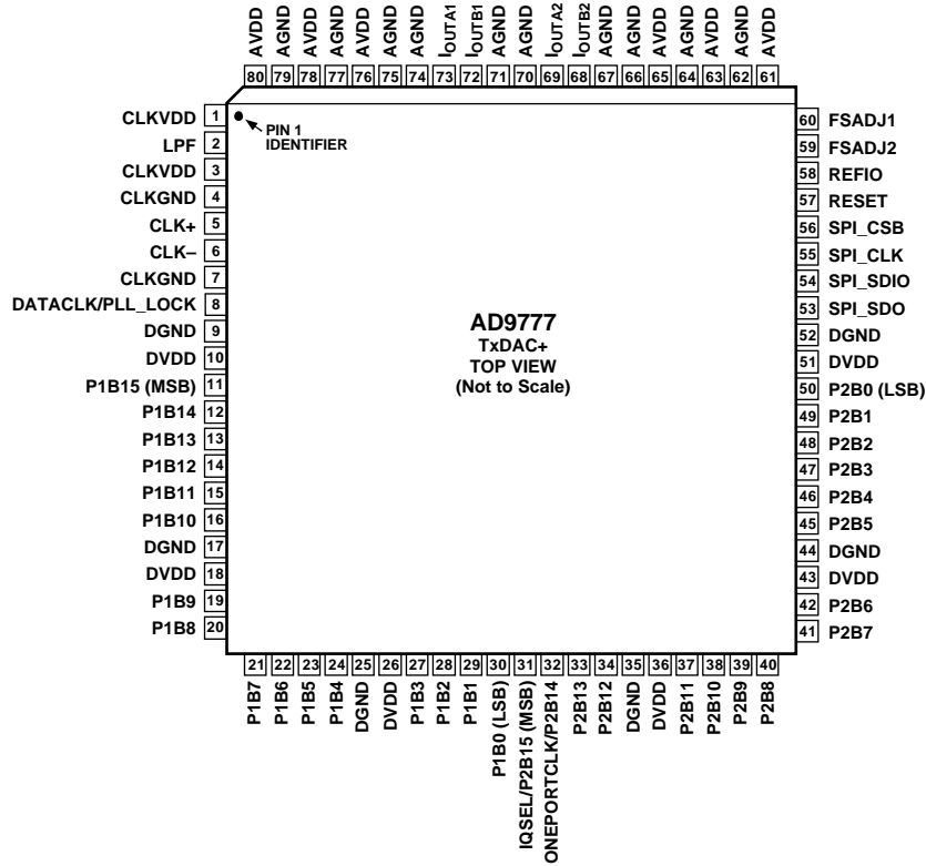
Figure 5. Pin Configuration
